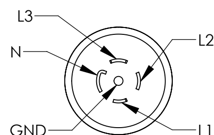
INPUT PLUG DETAIL NEMA L22-30P 30A / 5 COND
