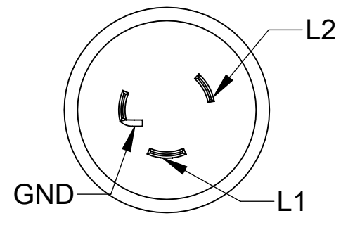
INPUT PLUG DETAIL NEMA L6-30P 30A / 3COND
