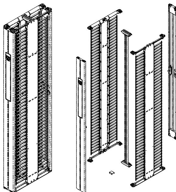
Motive Double-Sided Vertical Cable Manager P/N 32620-XXX
