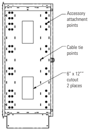
Rear Panel View (Interior Detail)
