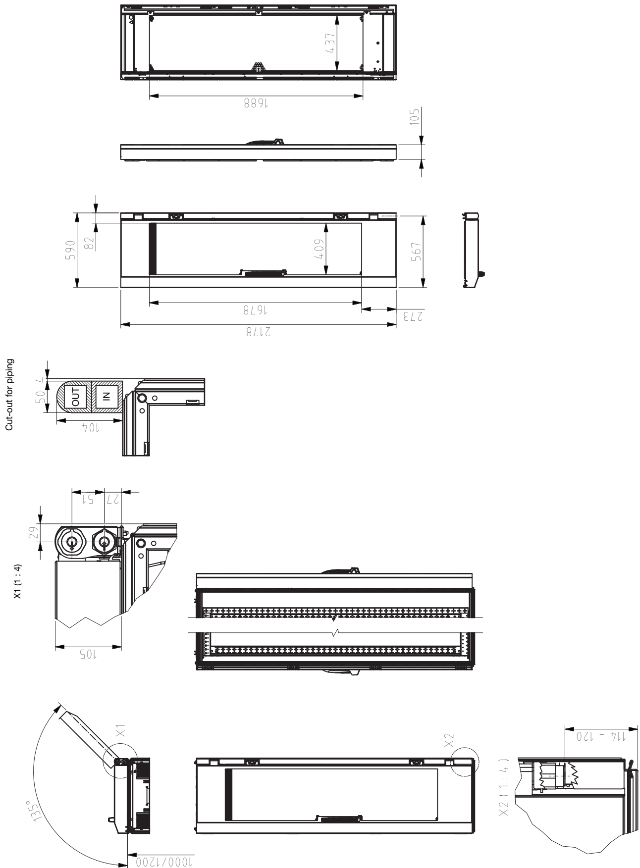
Fig. 34: Overview drawing of LCP Hybrid (600 x 2200)
