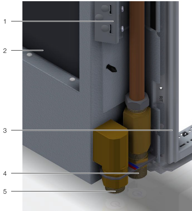
Fig. 8: Connection nozzles at the bottom of the LCP Hybrid
