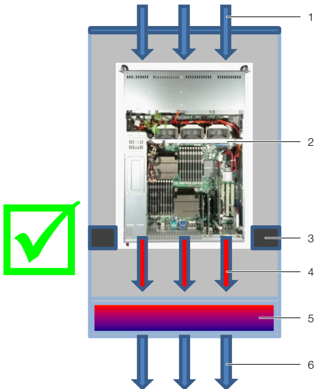
Fig. 3: Correct arrangement of the partitioning plates (air baffle plates)
