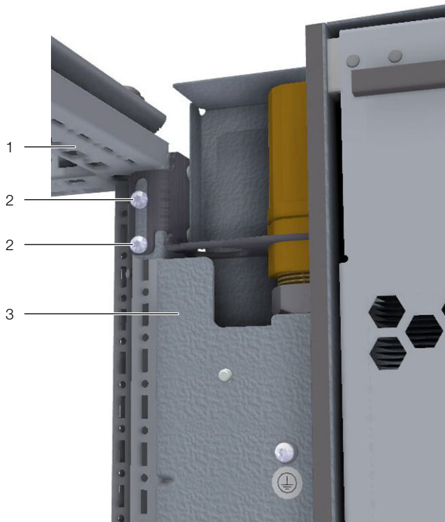
Fig. 16: Mounting the LCP Hybrid – Inside top
