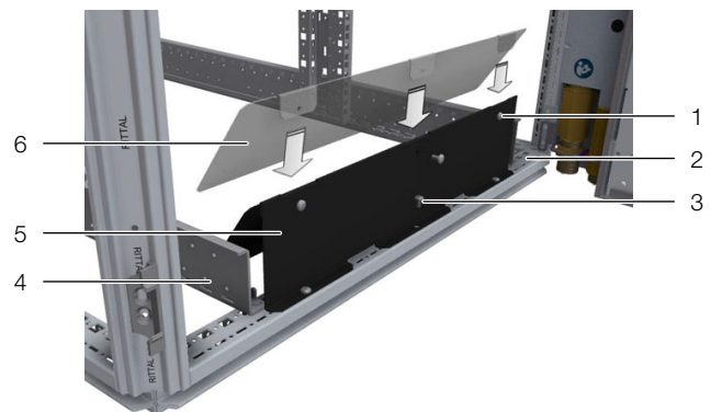
Fig. 18: Air routing kit at the bottom of the server enclosure
