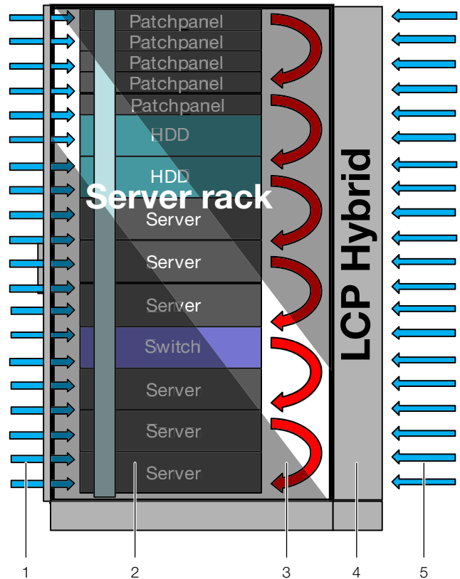
Fig. 10: Incorrect external air stream
