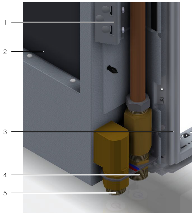
Fig. 20: Cold water network connection
