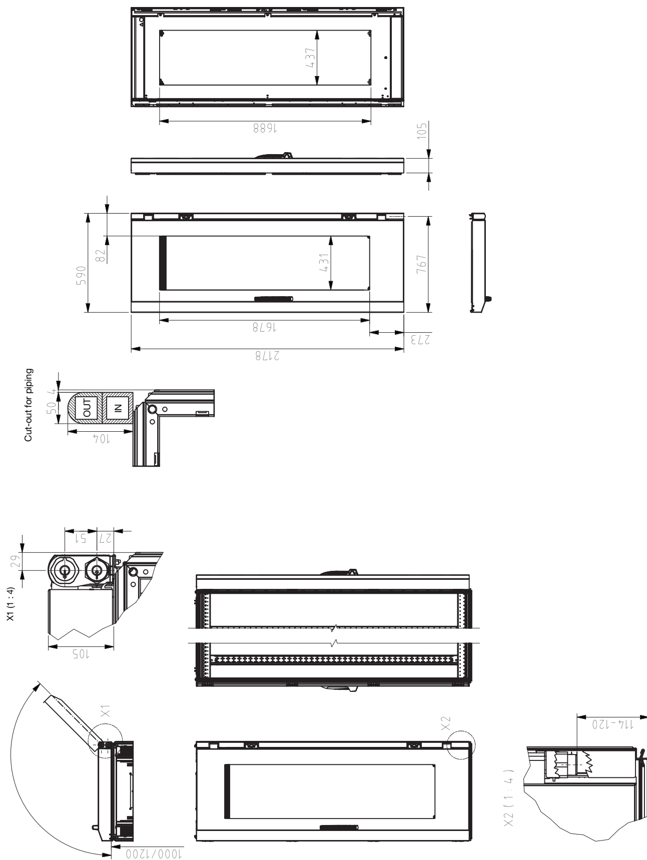
Fig. 35: Overview drawing of LCP Hybrid (800 x 2200)
