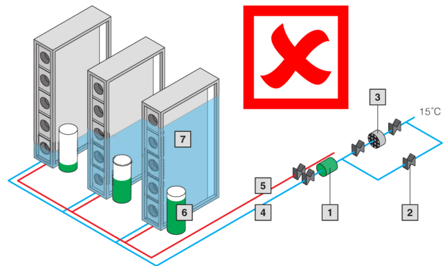
Fig. 21: Cooling distribution without hydraulic balancing
