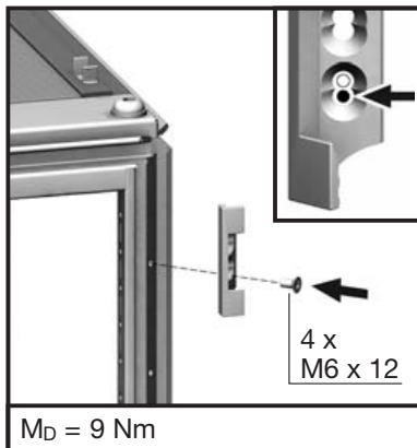
Fig. 14: Lock piece
