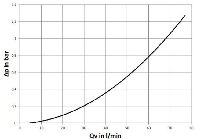
Fig. 30: Upstream pressure loss in the "10 kW" version
