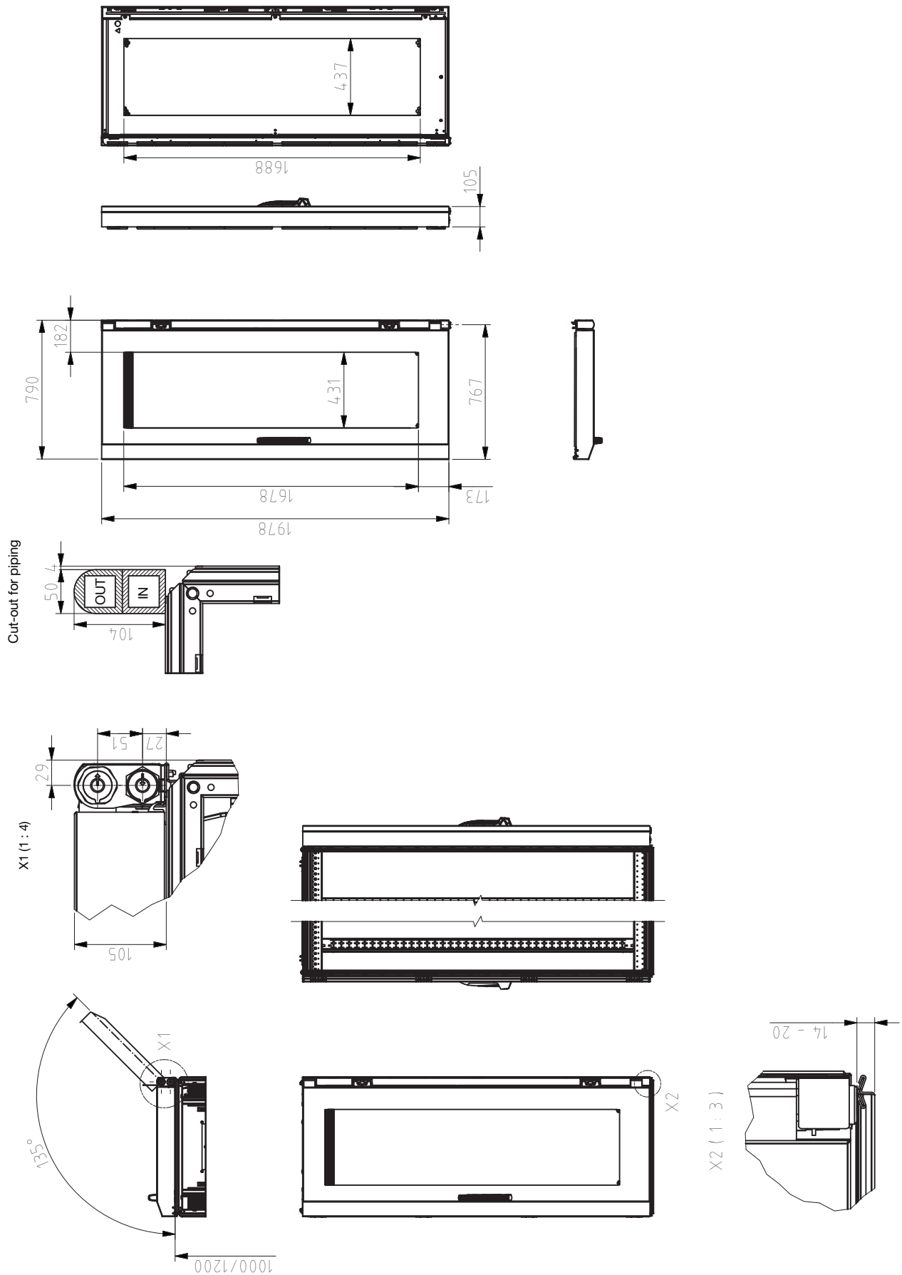
Fig. 33: Overview drawing of LCP Hybrid (800 x 2000)
