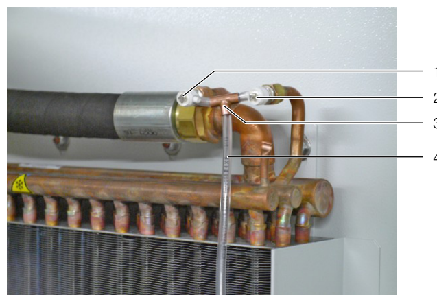
Fig. 25: Vent valves on the LCP Hybrid
