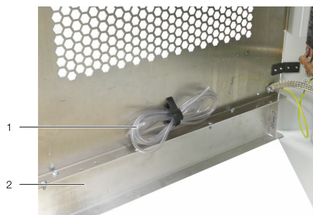
Fig. 24: Vent hose on the LCP Hybrid
