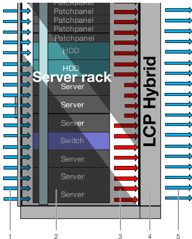
Fig. 1: Air routing on the LCP Hybrid – Side view
