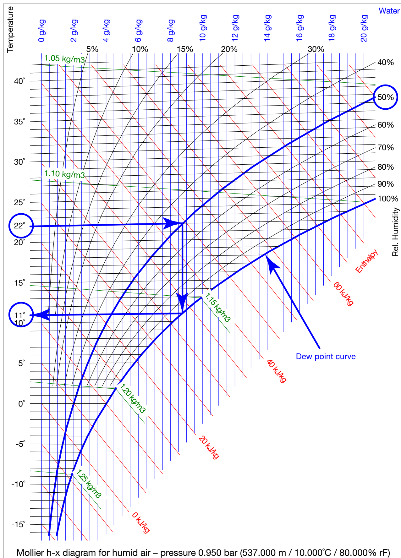
Fig. 2: Mollier h-x diagram for humid air
