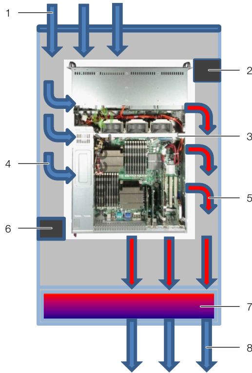
Fig. 5: Arrangement of the partitioning plates (air baffle plates) for devices with sideways air throughput
