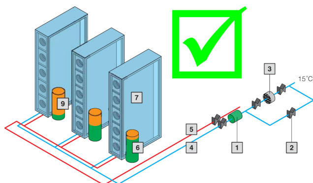
Fig. 23: Cooling distribution with Tichelmann principle
