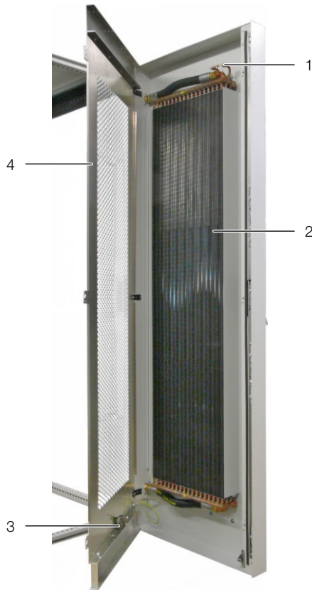
Fig. 7: LCP Hybrid – Maintenance door open
