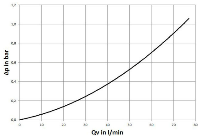
Fig. 31: Upstream pressure loss in the "20 kW" version
