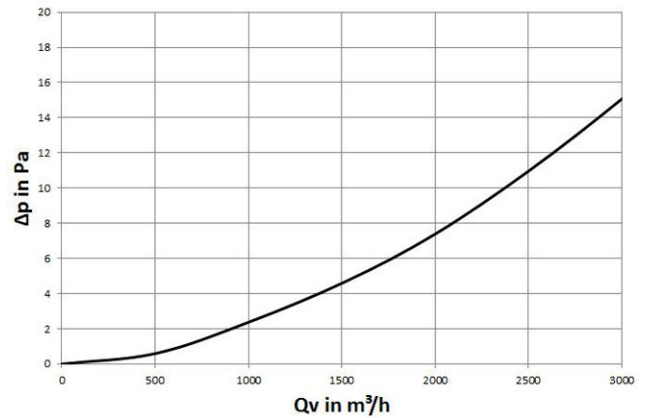
Fig. 28: Airside pressure loss in the "10 kW" version
