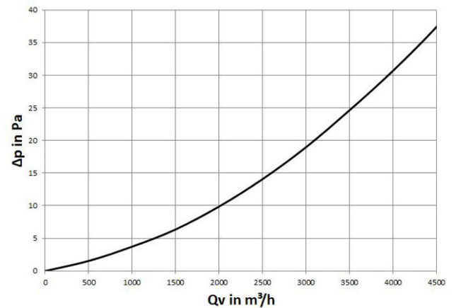
Fig. 29: Airside pressure loss in the "20 kW" version
