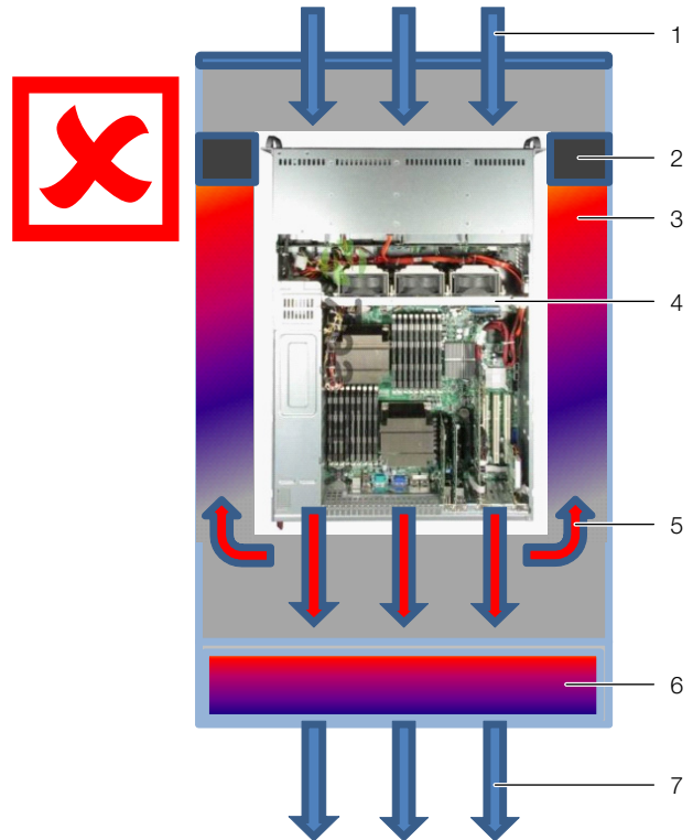
Fig. 4: Incorrect arrangement of the partitioning plates (air baffle plates)
