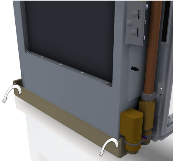
Fig. 19: Mounting aid on the LCP Hybrid
