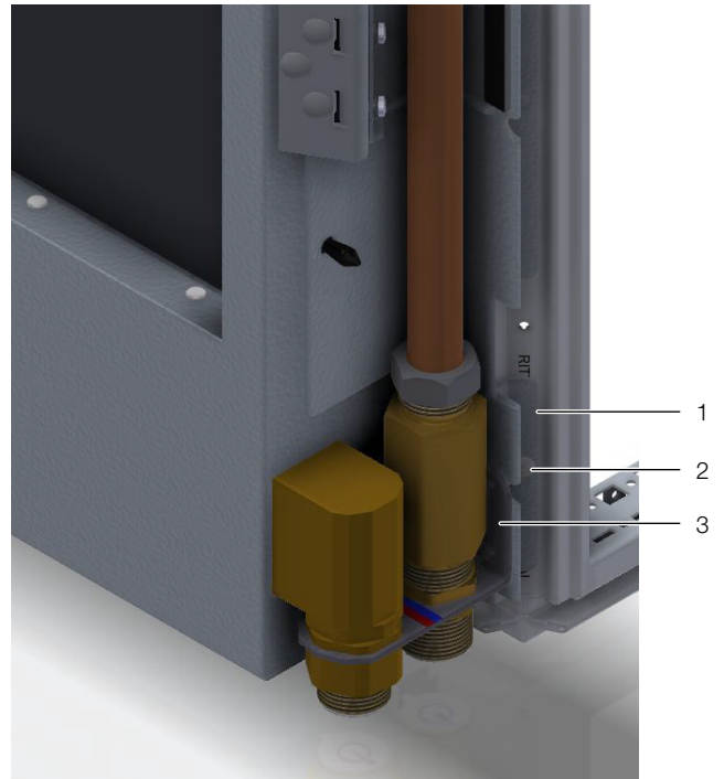
Fig. 15: Mounting the LCP Hybrid – Exterior
