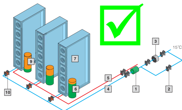
Fig. 22: Cooling distribution with hydraulic balancing
